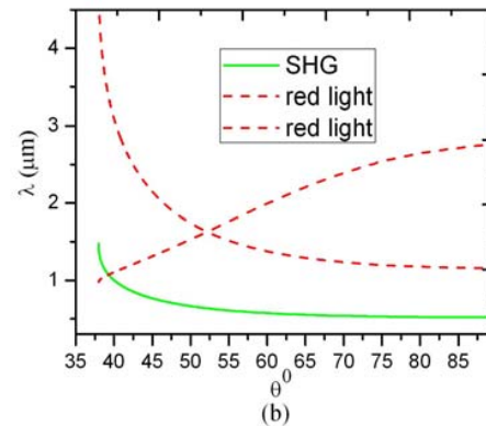
Fig. 6 (a) The spectra of the green light and red light; (b) Phase matching curves of KTA for the red light and SHG
