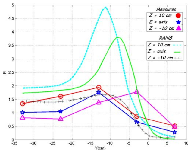
Fig. 14: Concentration profiles along the Y-axis (1000 rpm, X=25\text{cm} )
