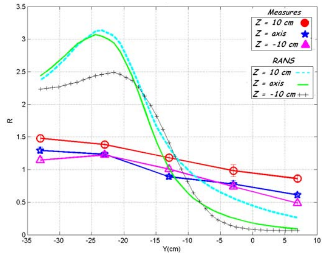
Fig. 16: Concentration profiles along the Y-axis (1000 rpm, X=50\text{cm} )
