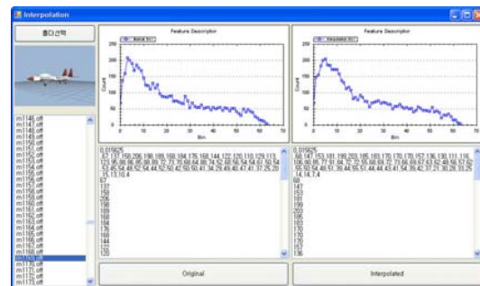
Fig. 5 Comparison original normal with interpolated normal
