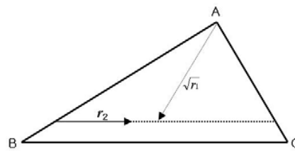
Fig. 3 Sampling a random point in a triangle
