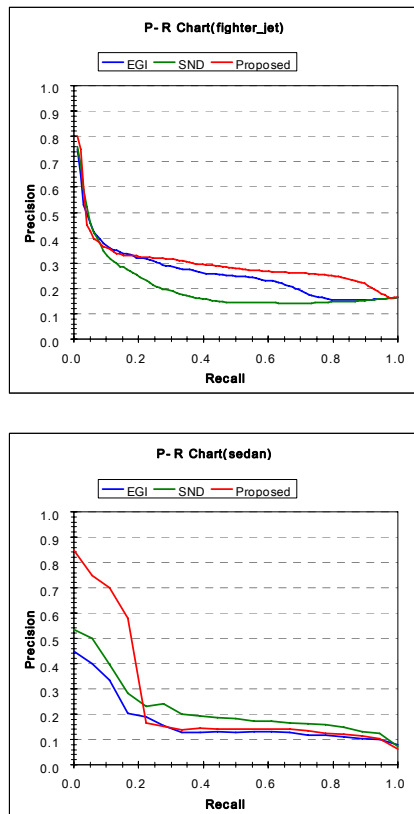
Fig. 7 Precision-Recall chart
