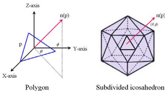
Fig. 4 Mapping from normals to the subdivided icosahedron
