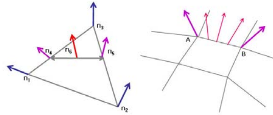
Fig. 2 Bilinear interpolations
