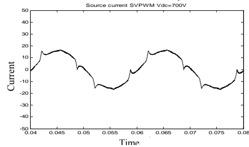
Fig.10.a. Source current wave form (SVPWM) V_{dc\ ref} = 700V
