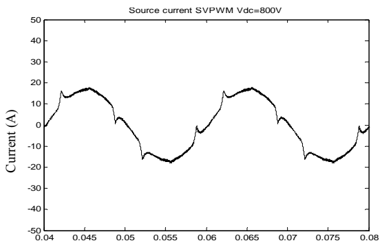
Fig. 12.a. Source current waveform (SVPWM) V_{dc\ ref} = 800V
