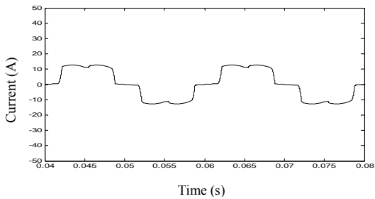
Fig. 9 (a) Load current waveform
