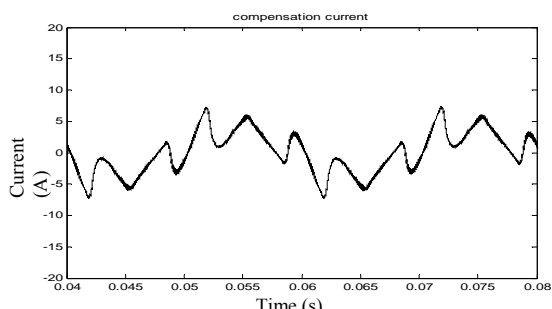
Fig.13.c. Compensation current waveform (SPWM) V dc ref= 800V
