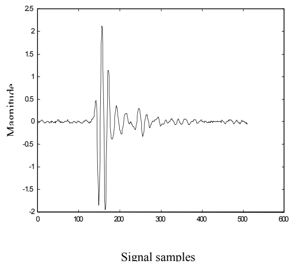
Fig. 5 DWT coefficients
