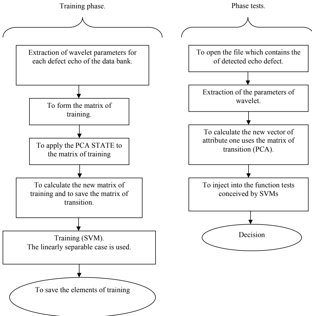
Fig. 3 The proposed algorithm
