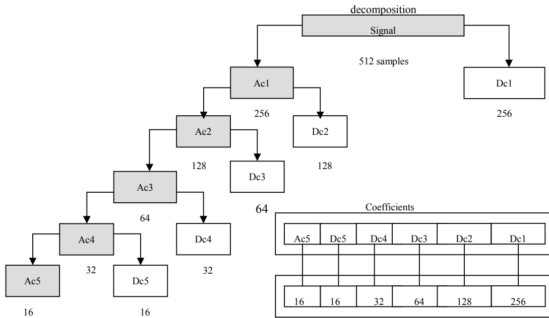
Fig. 1 Example of Wavelets coefficients calculation
