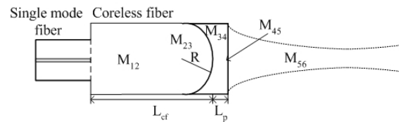
Fig. 1: The proposed fiber lens structure.
