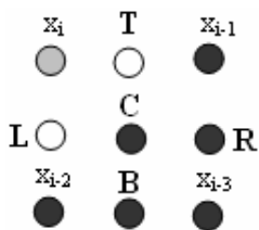
Fig. 14 A triangle with Top-Left corner edge
