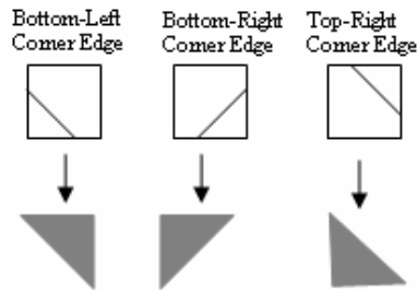
Fig. 7 Triangulations in a four-pixel square
