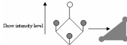
Fig. 6 Triangulation in a four-pixel square
