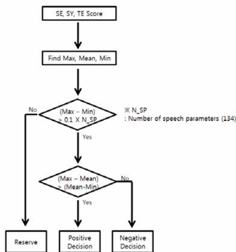
Fig. 5 The 3 decision types of the algorithm
