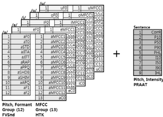
Fig. 1 Speech Features
