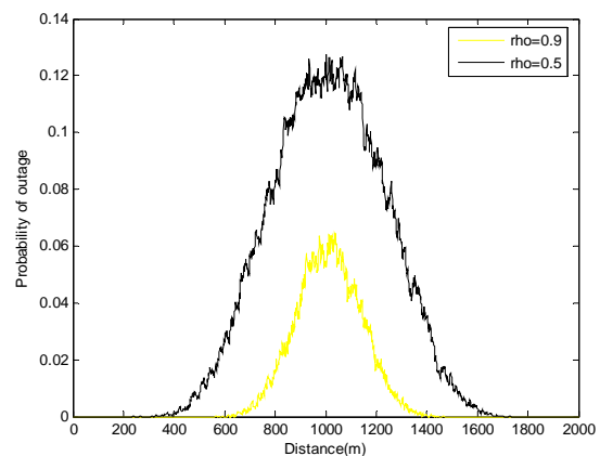
Fig. 5a Effect of Correlation coefficient (rho) on probability of outage for given \eta = 3.6, \sigma = 8dB, N = 20 .
