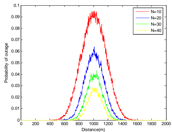
Fig. 2a Effect of window size on Probability of outage for given \rho = 0.5, \sigma = 8\text{dB}, \eta = 3.6
