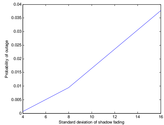
Fig. 4b Effect of standard deviation on probability of outage for given \eta = 3.6, \rho = 0.5, N = 20
