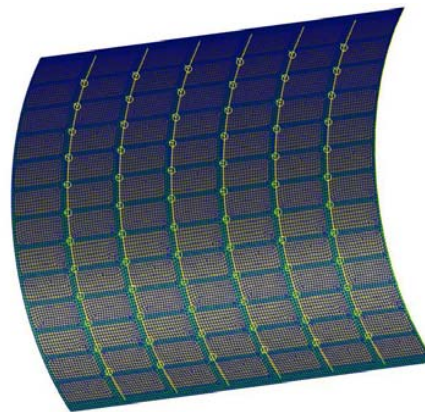
Fig. 3 Finite Element Model of Metallic skin panel structure
