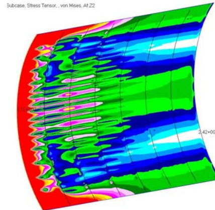
Fig. 10 Stress plot of composite skin panel under shear load
