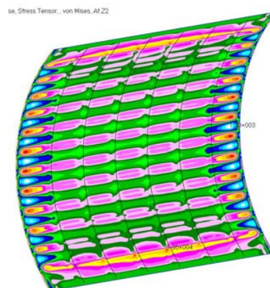
Fig. 4 Stress plot of metallic skin panel under decompression load
