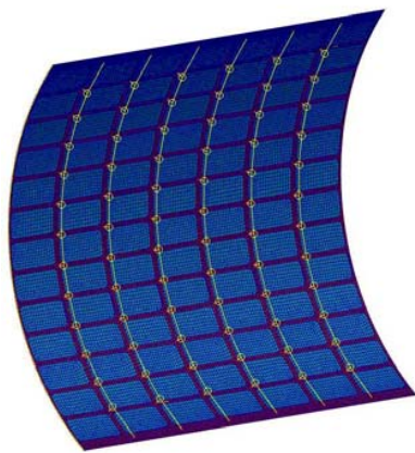
Fig. 8 Finite Element Model of Composite skin panel structure
