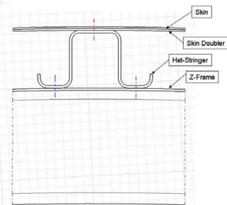
Fig. 2 Section view of metallic skin panel attachments
