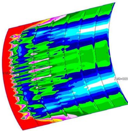
Fig. 5 Stress plot of metallic skin panel under shear load
