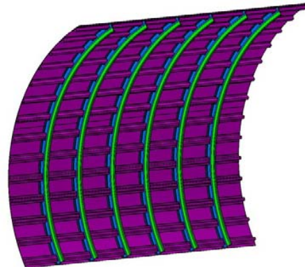
Fig. 6 CAD Model of Composite skin panel
