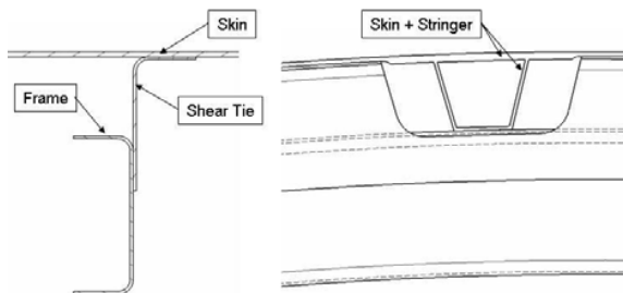
Fig. 7 Section view of composite skin panel attachments
