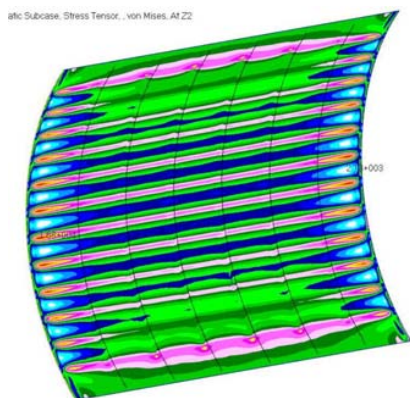
Fig. 9 Stress plot of composite skin panel under decompression load
