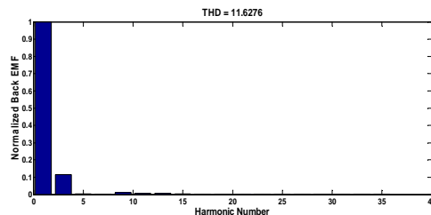
Fig. 12 Initial Harmonic Content (11.6276 %) for case 2
