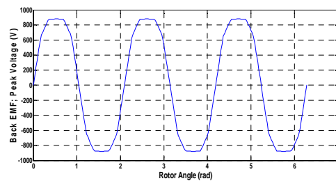
Fig. 20 Initial EMF Waveform
