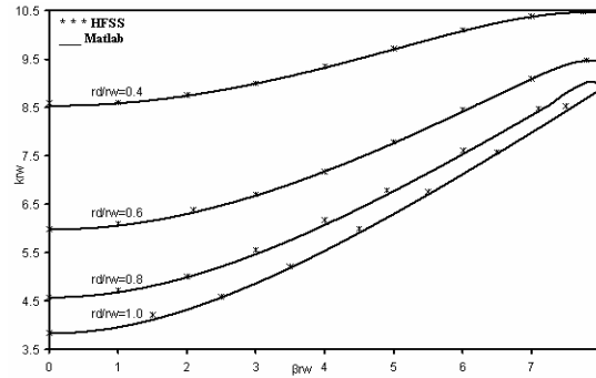
Fig. 2 Dispersion characteristic for a disc loaded waveguide operating in TE 01 mode having dimensions L/r_W = 0.4 and T/r_W = 0.1 , taking disc-hole radius as the parameter (solid curve), and validation against HFSS (shown by asterisks).
