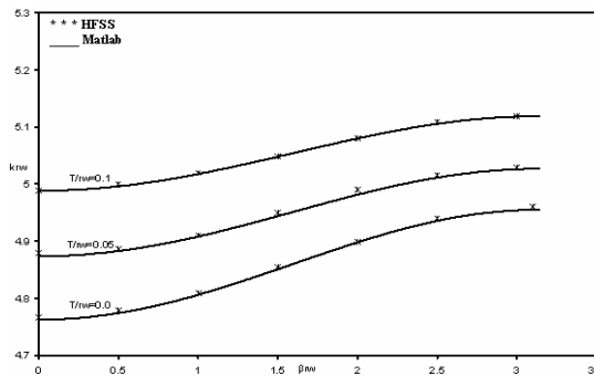
Fig. 4 Dispersion characteristic for a disc loaded waveguide operating in TE 01 mode having dimensions r_D/r_W = 0.5 and L/r_W = 1.0 , taking disc-thickness as the parameter (solid curve), and validation against HFSS (shown by asterisks).
