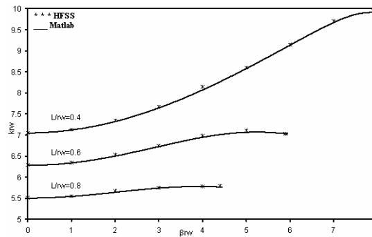
Fig. 3 Dispersion characteristic for a disc loaded waveguide operating in TE 01 mode having dimensions r_D/r_W = 0.5 and T/r_W = 0.1 , taking disc-periodicity as the parameter (solid curve), and validation against HFSS (shown by asterisks).
