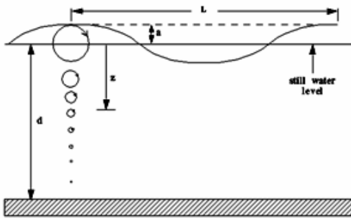
Fig. 1 Wave particle motion in deep water [12]
