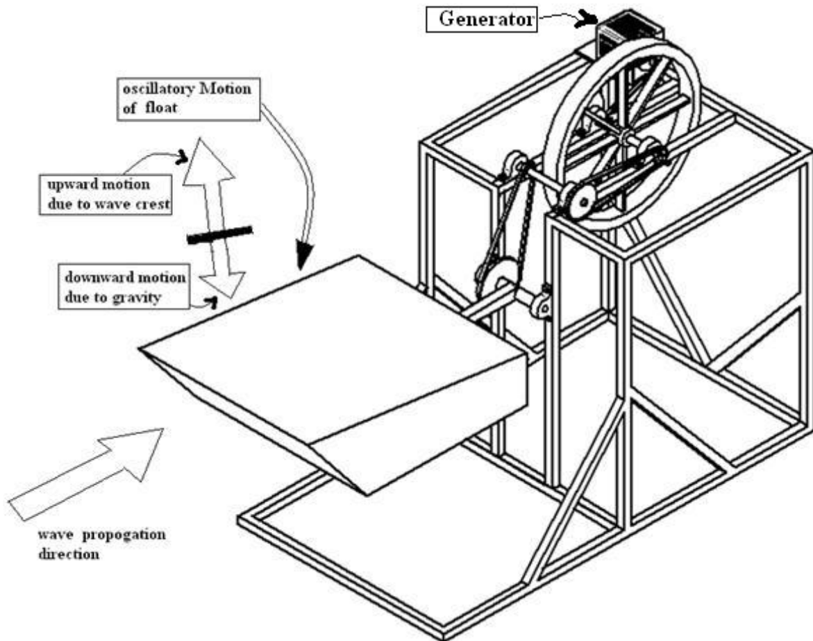
Fig. 9 Complete assembly of SAS-2
