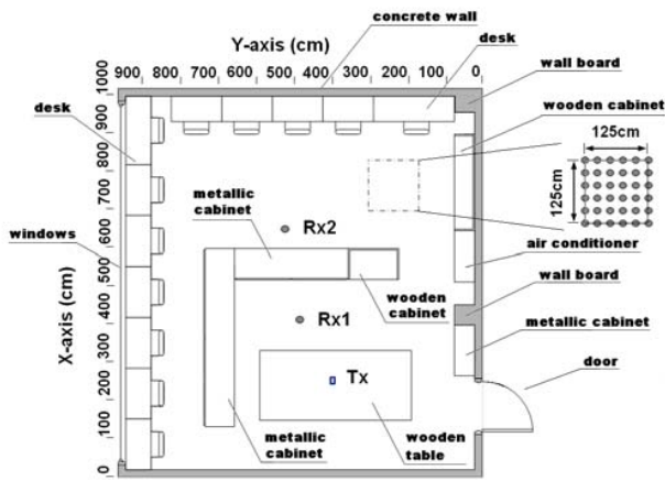
Fig. 2 Top view of the Microwave laboratory in Tamkang University and this laboratory has dimensions of 9.2m (Length) x 10m (Width) x 3m (Height). The transmitter is located at Tx (250, 400, 120) cm, the receiver are located at Rx1 (400, 500, 75)cm and Rx2 (650, 525, 75)cm
