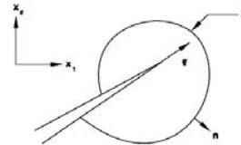
Fig. 4 Contour for calculating J-integral
