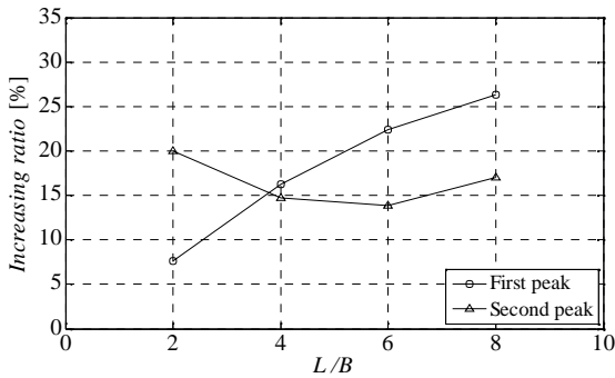
Fig. 11 Increasing heat transfer ratio at H/B=15, L_1/B=4
