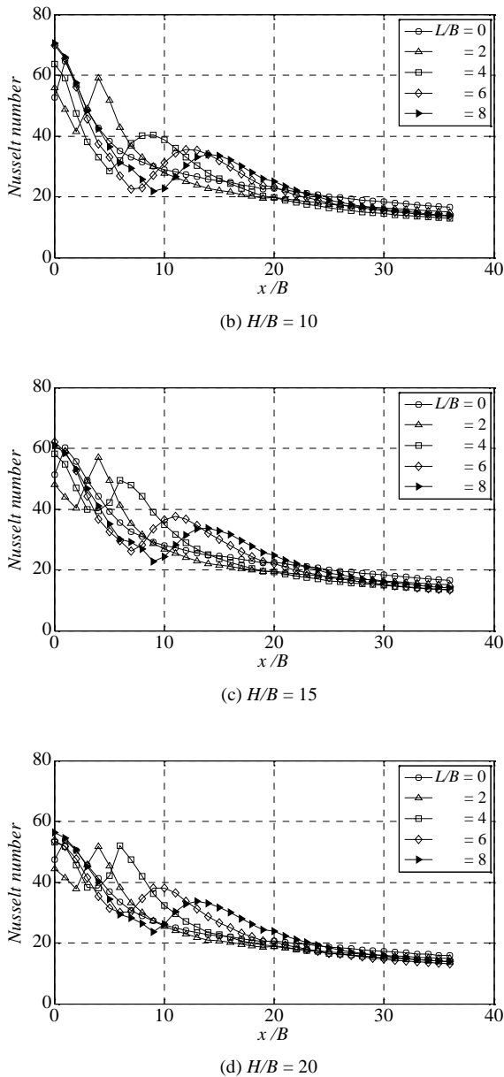
Fig. 7 Nusselt number distribution with single rib
