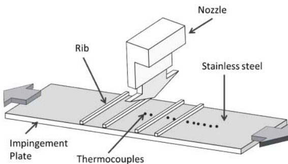
Fig. 2 Schematic diagram of the rib wall
