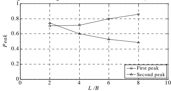
Fig. 12 Normalized peak value at H/B=15, L_1/B=4
