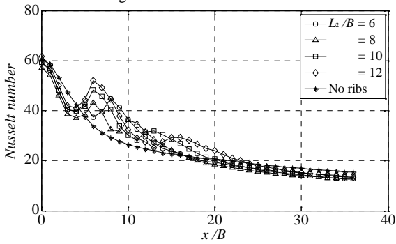
Fig. 10 Nusselt number distribution at H/B=15, L_1/B=4
