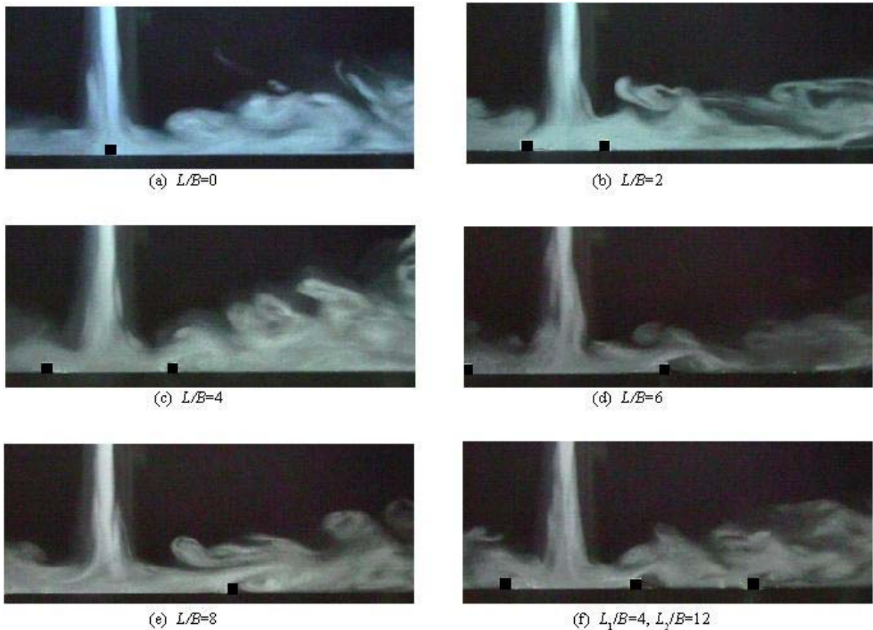
Fig. 12 Flow visualizations at H/B=15
