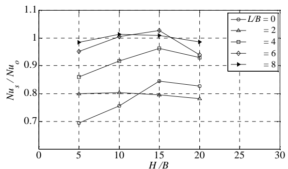
Fig. 8 Nusselt number at the stagnation point
