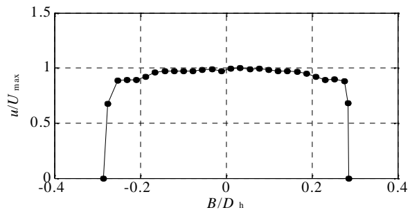
Fig. 5 The mean velocity
