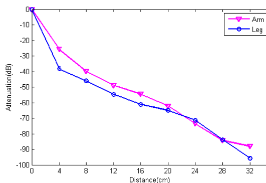
Fig. 4 Signal attenuations are shown with respect to distance. Two cases of arm and leg are measured
