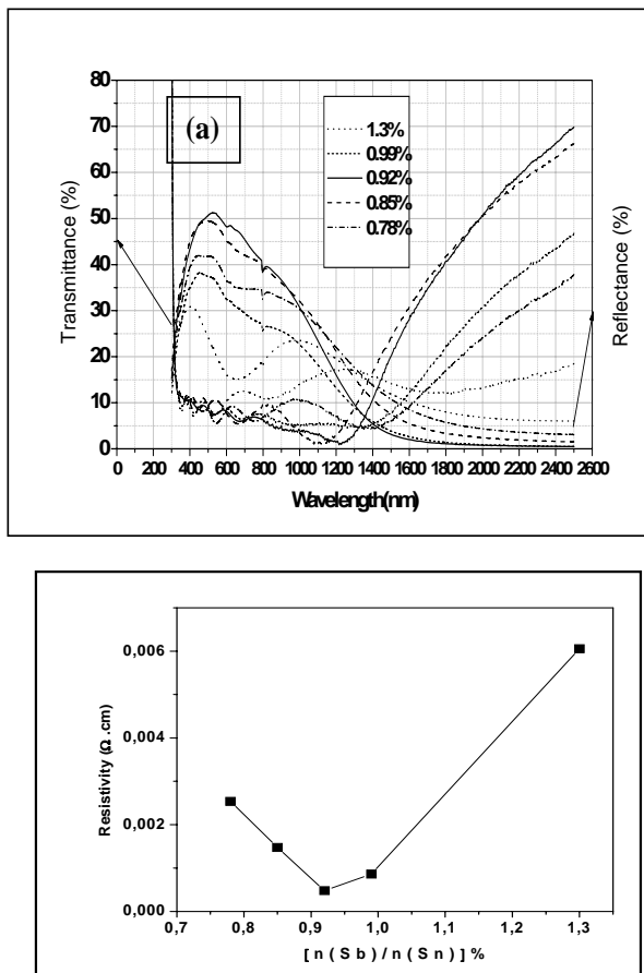
Fig. 4 Transmittance, reflectance a) and resistivity b) upon [\text{n}(\text{Sb})/\text{n}(\text{Sn})] % concentration respectively, ( T_s=443^\circ\text{C} , \text{O}_2 : 2 L/min) showing that the best resistivity correspond to the weakest reflectance
