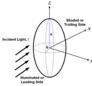
Fig. 1. Physical model of a prolate spheroid photophoresis
