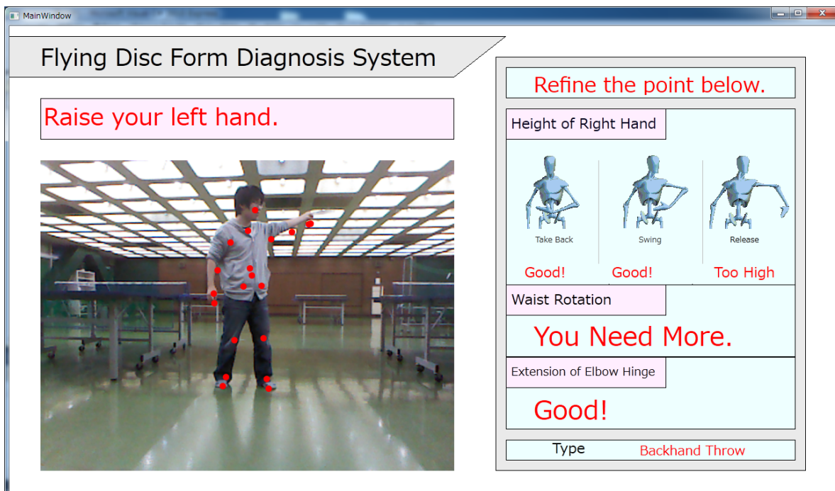
Fig. 3 Sample Screenshot
