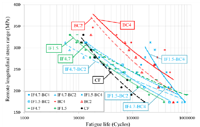
Fig. 2 S-N curve of experimental fatigue tests [9]
