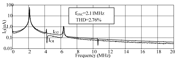
Fig. 5 Frequency spectrum of signal in Fig. 4
