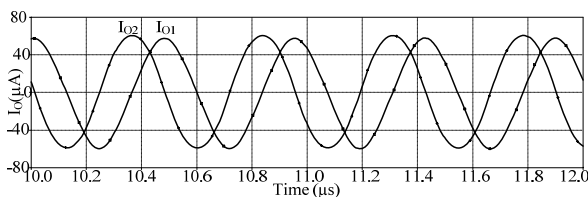
Fig. 4 The simulation result of quadrature outputs
