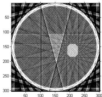
Fig. 7c 15 degree 12 profiles
