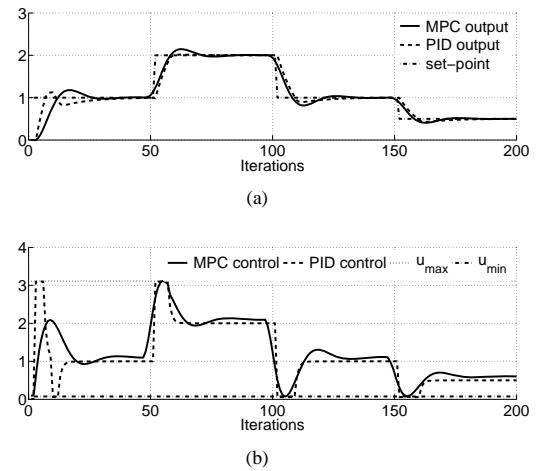
Fig. 3. Closed-loop simulation results for the first order plant
