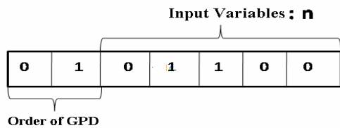
Fig. 2 Structure of binary chromosome
