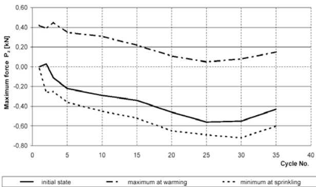
Fig. 10 Maximum force at points E, F, along the z-axis
