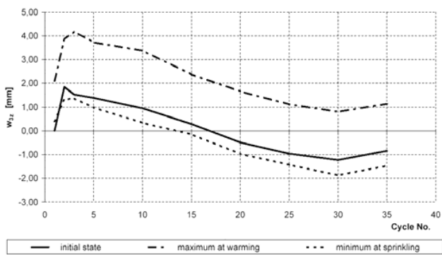
Fig. 11 Deflection at central point 3 along z-axis
