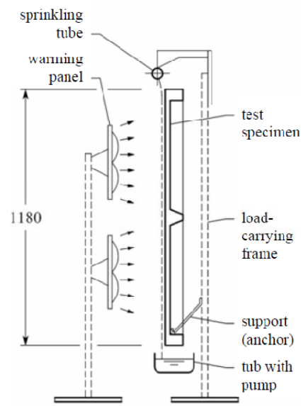
Fig. 1 Scheme of test equipment
