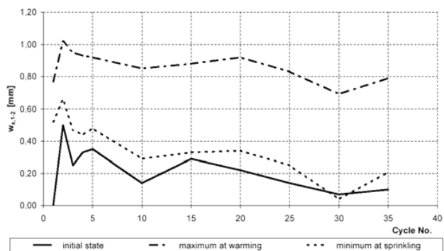
Fig. 12 Entire elongation between points 1 and 2
