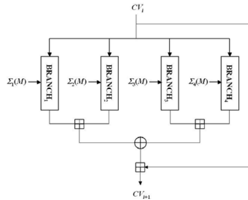
Fig. 1 Outline of the FORK-256 compression function
