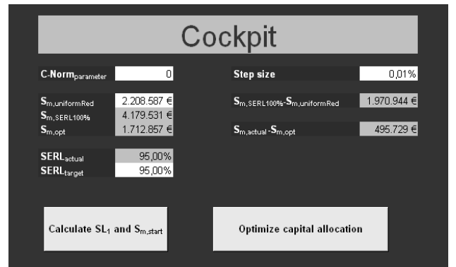
Fig. 6 Software interface
