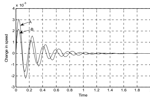
Fig. 11 Dynamic response of \Delta\omega for STATCOM with additional power oscillation damping controller for different values of X_e
