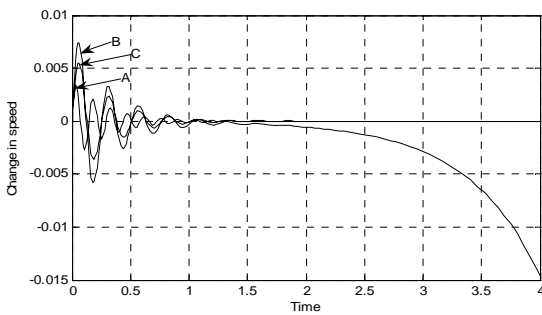
Fig. 7 Dynamic response for \Delta\omega
