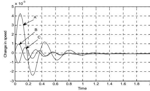
Fig. 10 Dynamic response for \Delta\omega for different values of
