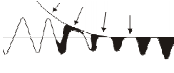
Fig. 1 Burnishing Process
