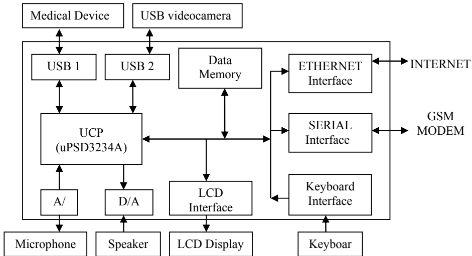
Fig. 2 The biosignal / ECG telemonitoring unit of our project
