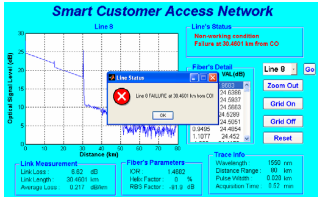
Fig. 11 Another example of failure line in the Line's Detail window for two events
