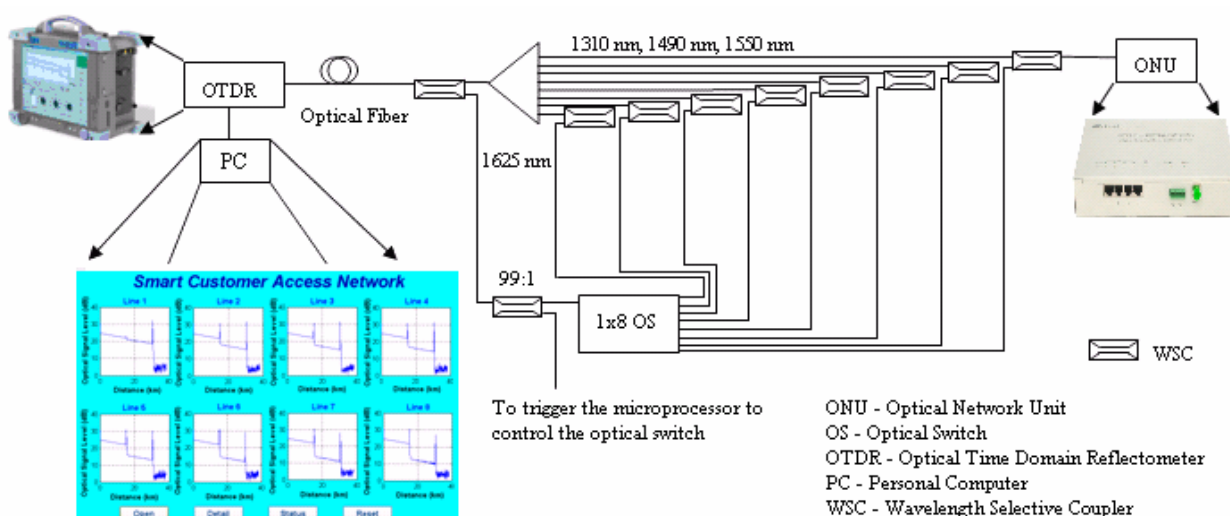
Fig. 3 Centralized monitoring and self-protected against fiber fault in FTTH using SANTAD in the downstream direction
