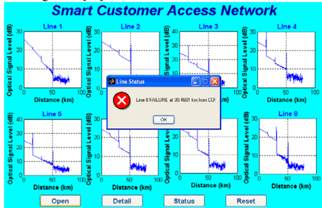
Fig. 7 A failure message displays to show the faulty line and failure location in the FTTH network system
