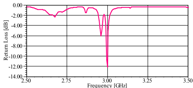
Fig. 6 Return loss of the proposed patch antenna
