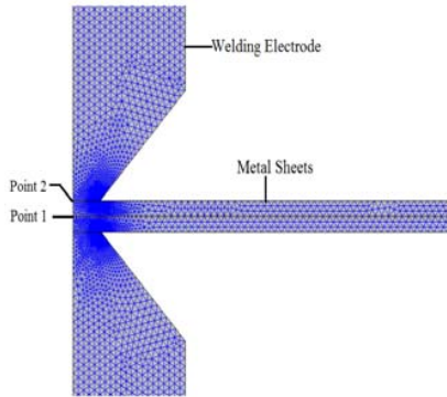
Fig. 2 Geometry meshing
