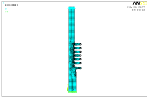
Fig. 3 Boundary Conditions
