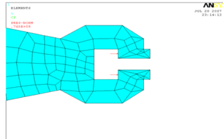
Fig. 8 Pressure applied at the Rotor Groove
