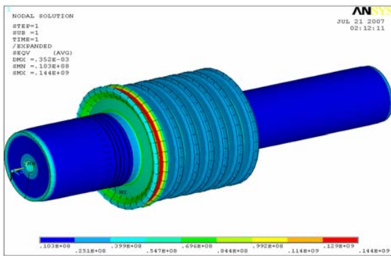
Fig. 14 Symmetry Expansion Plot
