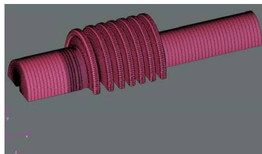
Fig. 2 FE Modeling of Half of the Steam Turbine Rotor
