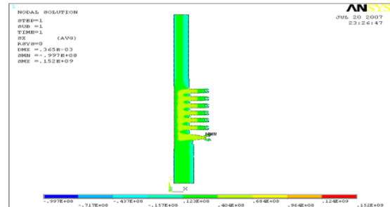
Fig. 9 Radial Stress
