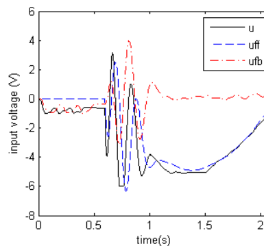
Fig. 9 Control input signal from FEL controller to motor A
