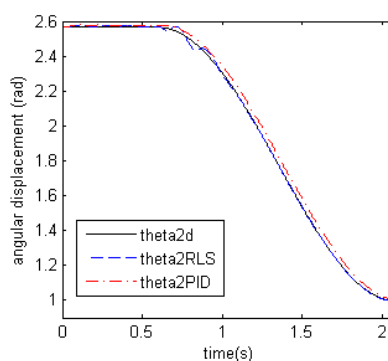
Fig. 8 Angular displacement of link 2, \theta_2 under PID and FEL control
