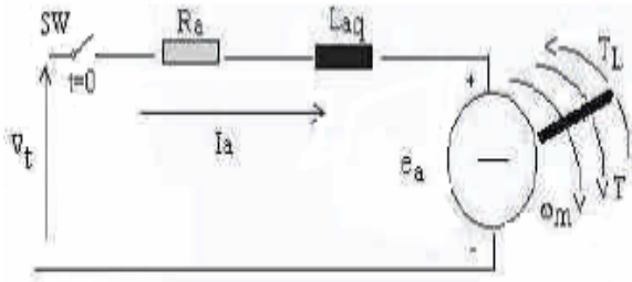
Fig. 1 Schematic Diagram of a DC Motor [6]
