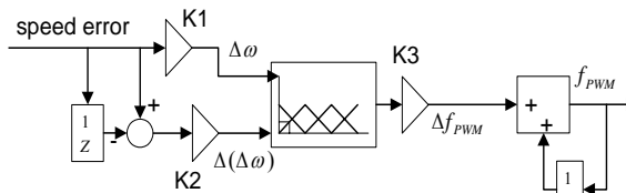
Fig. 2 Block diagram of PI fuzzy logic controller
