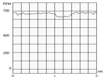
Fig. 7 Load-changing response
