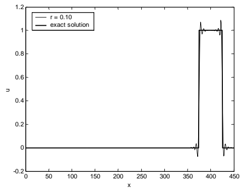
Fig. 11b Propagation of Boxcar function at dimensionless time, t=400 at cfl 0.10 using the spatial scheme proposed by Lockard et al. coupled with the optimized time discretisation designed by Tam and Webb
