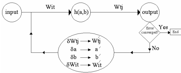
Fig. 7 the WNN training cycle
