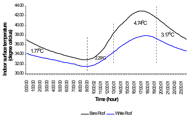
Fig. 9 (c): Comparison of average indoor surface temperature between black bare roof and white roof for six days' reading
