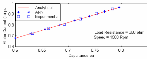
Fig. 10 Variation of stator current with capacitance
