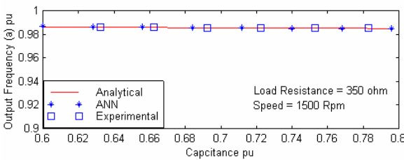
Fig. 8 Variation of output frequency with capacitance
