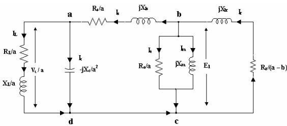
Fig. 1 Conventional equivalent circuit of SEIG without active voltage source
