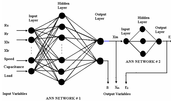
Fig. 5 Cascaded artificial neural network
