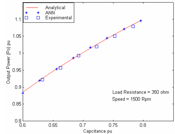
Fig. 11 Variation of output power with capacitance
