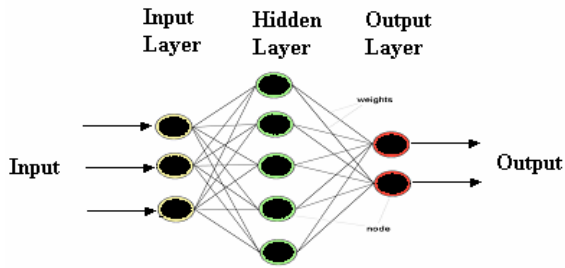
Fig. 4 Architecture of multilayer perceptron
