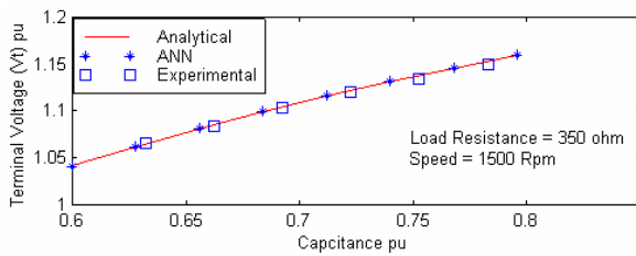
Fig. 7 Variation of terminal voltage with capacitance
