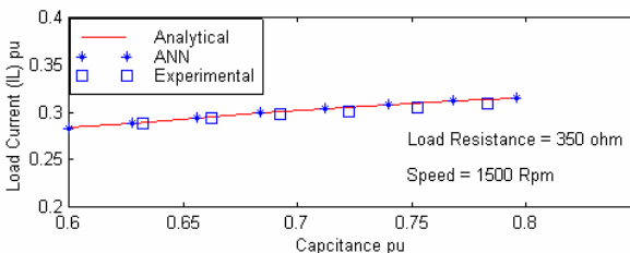
Fig. 9 Variation of load current with capacitance
