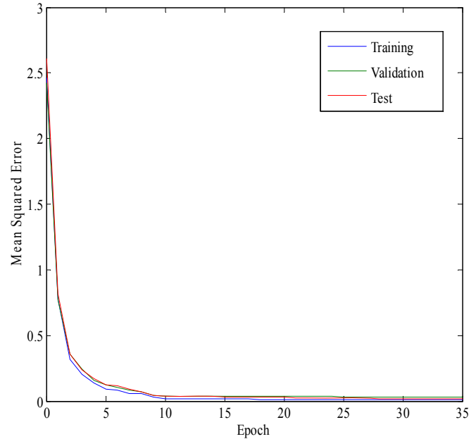
Fig. 3 Training, validation and test mean squared errors for the Levenberg-Marquardt algorithm
