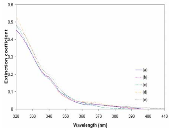
Fig. 6 Extinction coefficient of \text{TiO}_2 films: (a) as-grown at room temp. (b) annealed at 300 °C, (c) 400 °C, (d) 500 °C and (e) 600 °C
