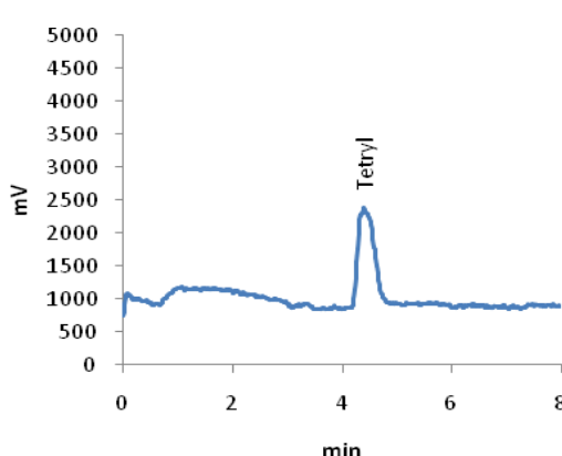
Fig. 5 Chromatogram of standard solution of Tetryl 3.5 \times 10^{-7} M
