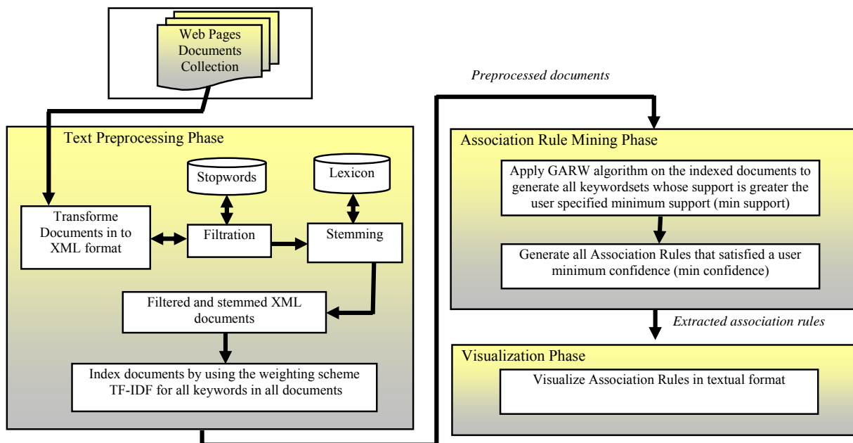
Fig. 1 Text Mining System Architecture
