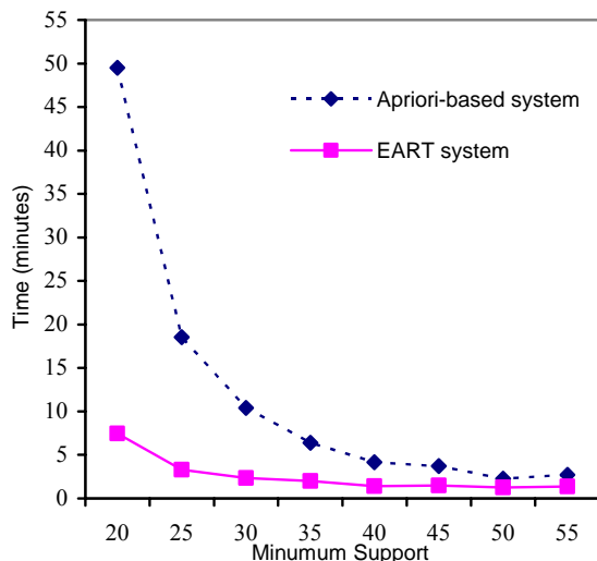
Fig. 5 EART system Vs Apriori-based system
