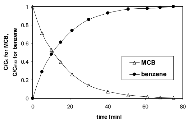
Fig. 1 Batch hydrodechlorination of MCB to benzene on Pd/Al 2 O 3 in clean deionized water. Reaction conditions: c_{0,MCB} = 20 \text{ mg L}^{-1} , c_{Pd} = 0.75 \text{ mg L}^{-1}
