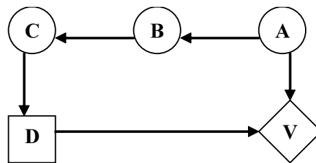
Fig. 1. An example of influence diagram
