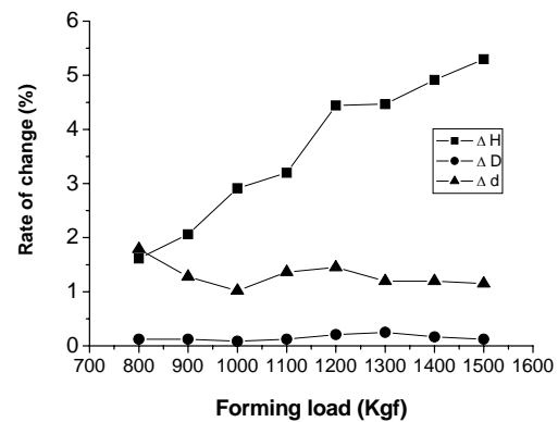
Fig. 9 Difference of dimension after the forming
