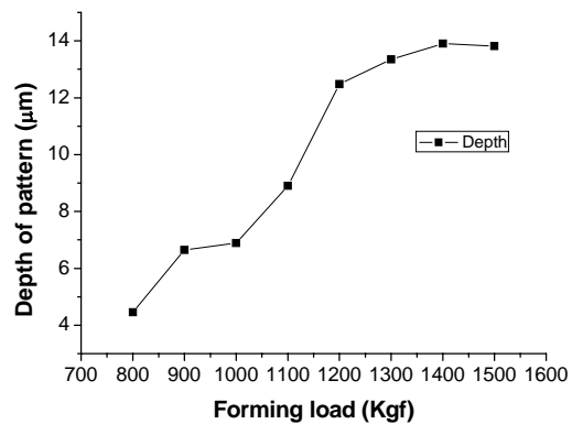
Fig. 10 Experiment result with various forming load
