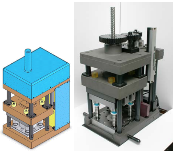
Fig. 3 Desktop forming system
