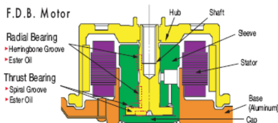
Fig. 1 Structure of the fluid dynamic bearing
