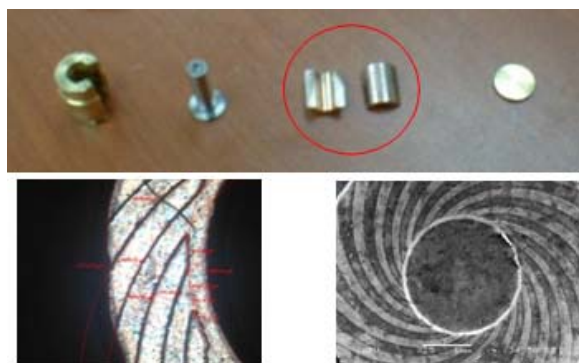
Fig. 2 Spiral patterns on the FDB used in 3.5 inch HDD
