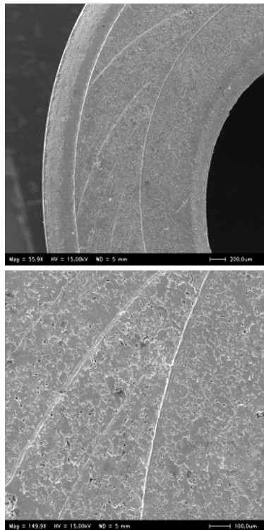
Fig. 11 Top-view SEM of FDB (forming load:1, 400Kgf)
