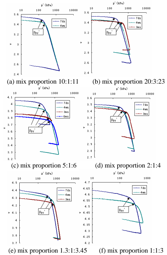
Fig. 3 Isotropic compression behaviors for specimens with different mix proportion and curing time
