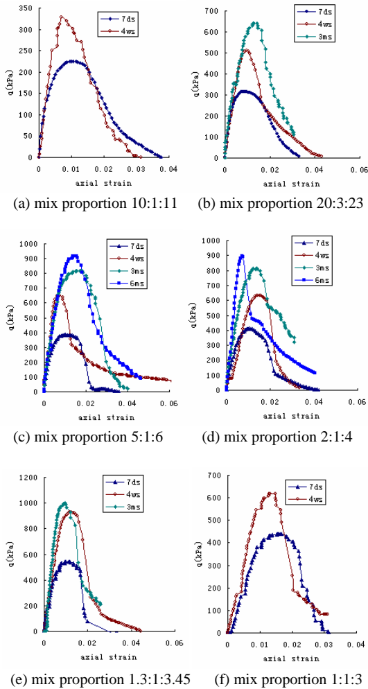
Fig. 2 Unconfined compressive strength for specimens with different mix proportion and curing time
