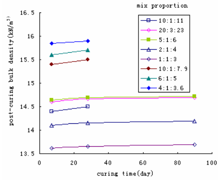
(a) post-curing bulk density versus curing time
