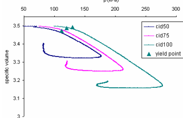
(c) compression space under CID test
